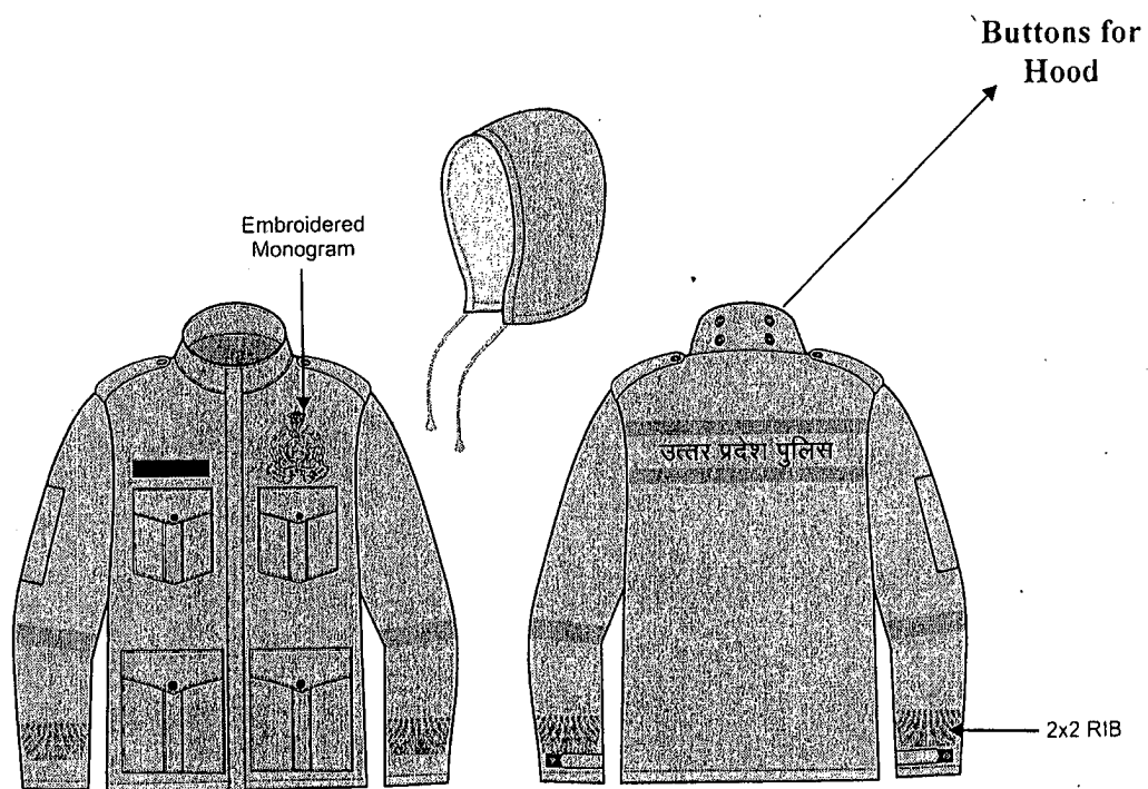
BASIC PATTERN OF JACKET
